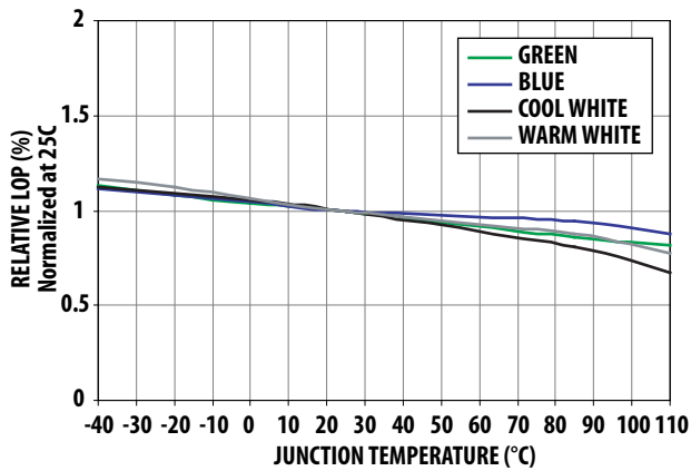
Figure 15. Relative LOP vs. junction temperature for InGaN
